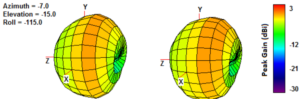
Figure 7. 3D Radiation Pattern at 850 MHz (left) 915 MHz (right) of the TG19 Antenna.
