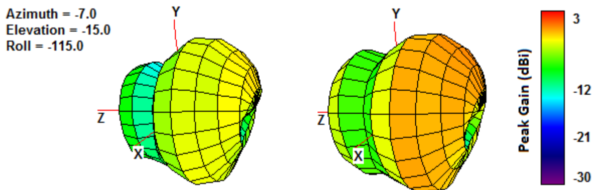
Figure 8. 3D Radiation Pattern at 1710 MHz (left), 1805 MHz (right) of the TG19 Antenna.
