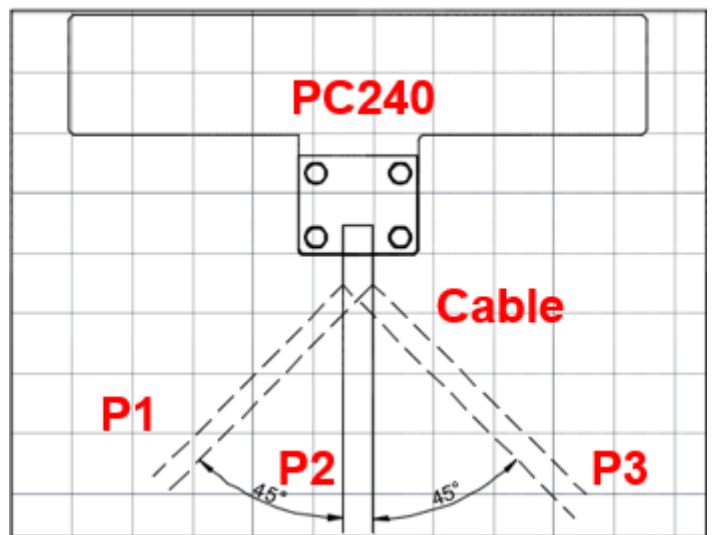
Cable Routing
