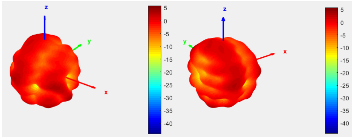
Radiation Pattern @ 6.5GHz
