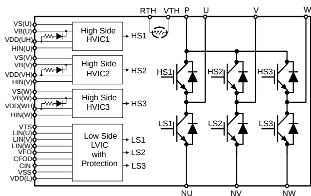
Figure 1. Application Schematic
