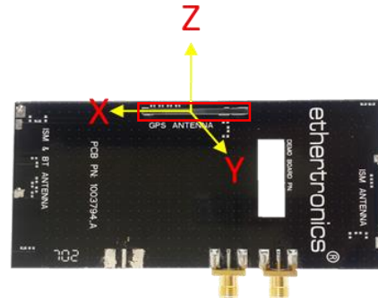
Single Band antenna (GPS Layout Orientation)
