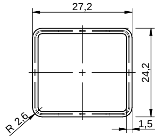
0,5mm Recommended Tin Paste Mask Layer
