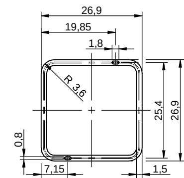
0,5mm Recommended Tin Paste Mask Layer
