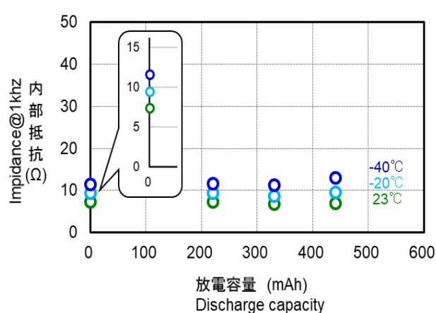
Impedance by Temperature
