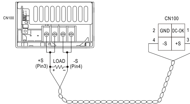
Fig 2.1 Sense lines should be twisted in pairs
