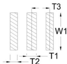
Figure 3) Land Pattern
