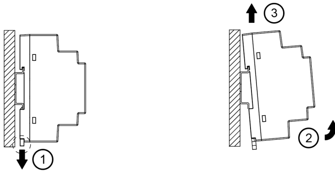
Fig. 2.2 Dismounting
