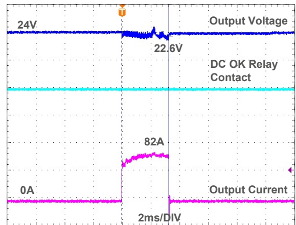
Fig. 8.2 APB 400% of nominal output current for 2ms
