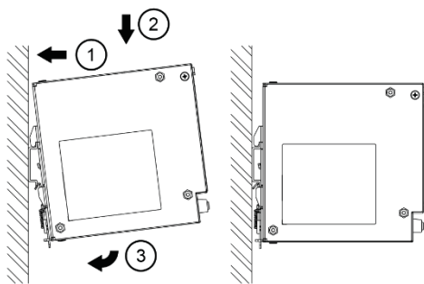
Fig. 6.1 Mounting
