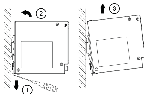
Fig. 6.2 Dismounting
