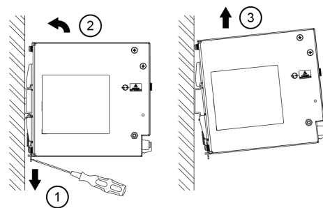
Fig. 6.2 Dismounting
