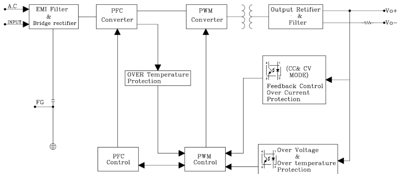
DRL-24V480W1AA
