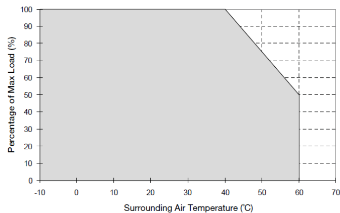
Fig.1.2 De-rating for Mounting Orientation A to F > 40°C de-rate power by 2.5% / °C
