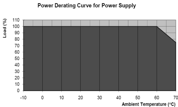
Fig. 1 De-rating for Vertical and Horizontal Mounting Orientation > 60°C de-rate power by 2.5% / °C
