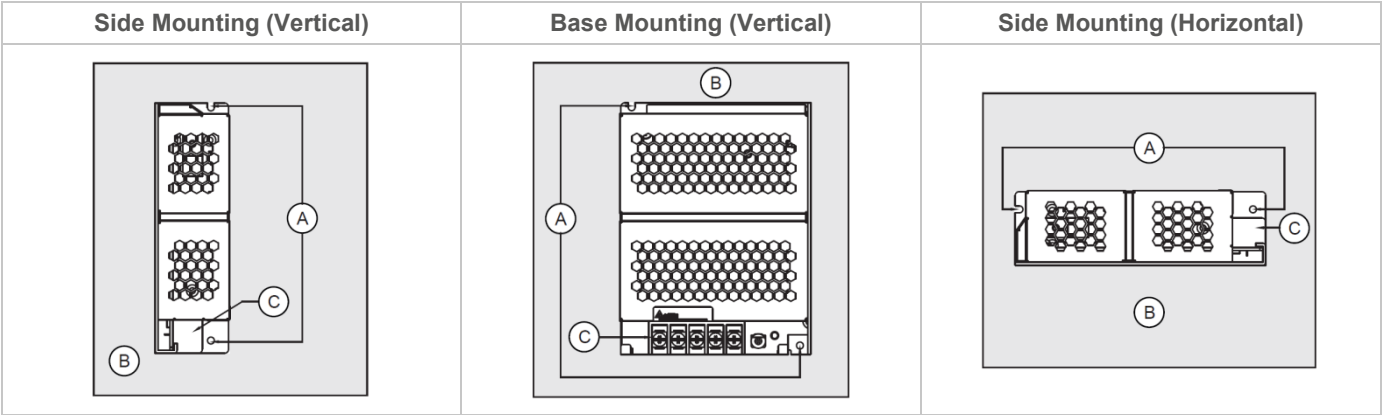
Fig. 2 Recommended Mounting Orientations
