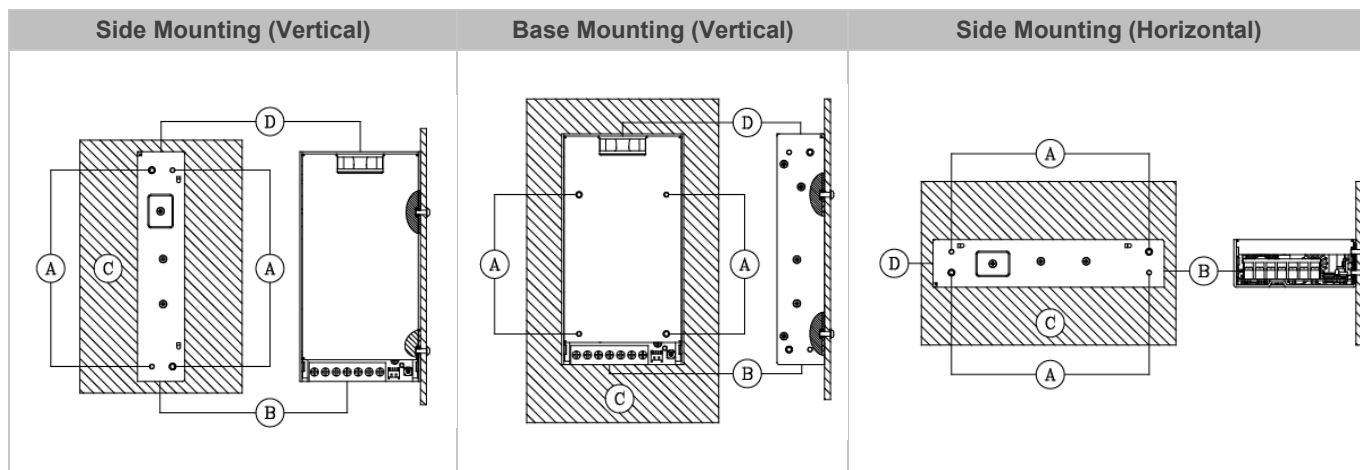
Fig. 2 Mounting Orientation
