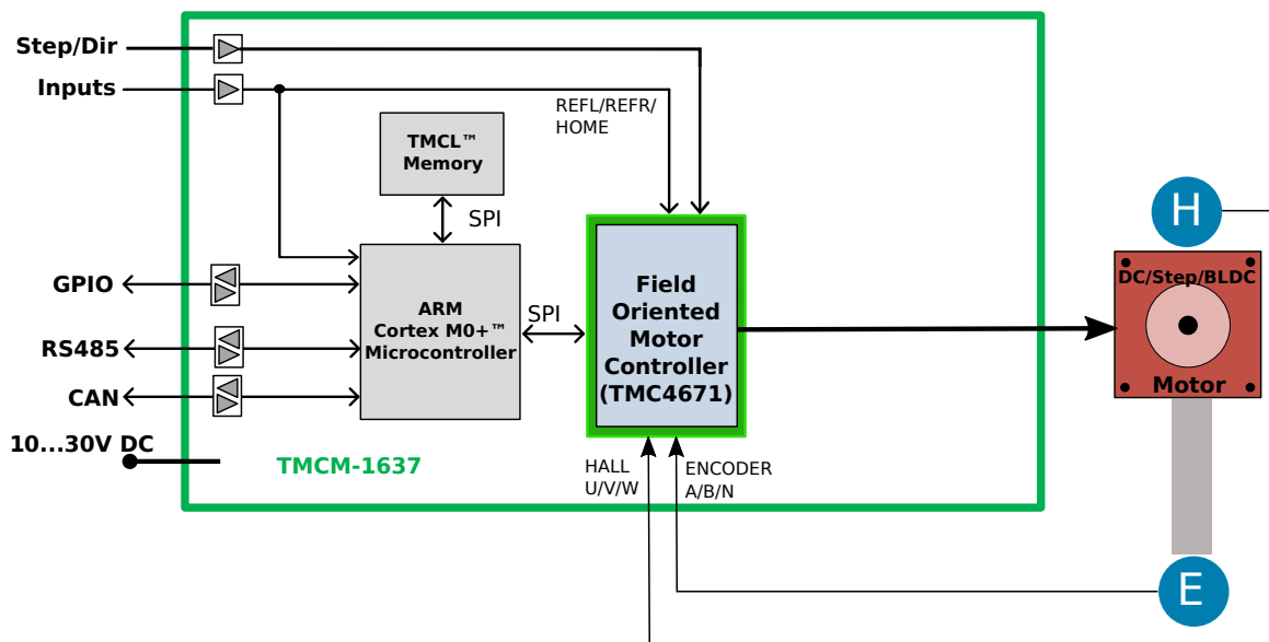
Figure 7: TMC1637 block diagram
