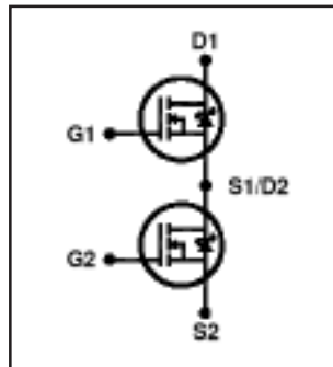
TO-220 Full-Pak 5 PIN
