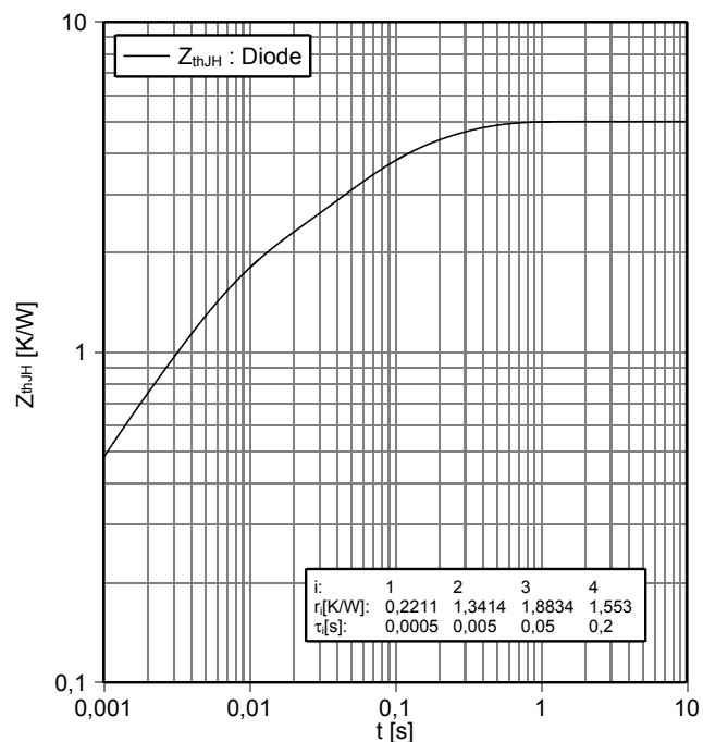
瞬态热阻抗 二极管, 三电平 transient thermal impedance Diode, 3-Level Z_{thJH} = f(t)
