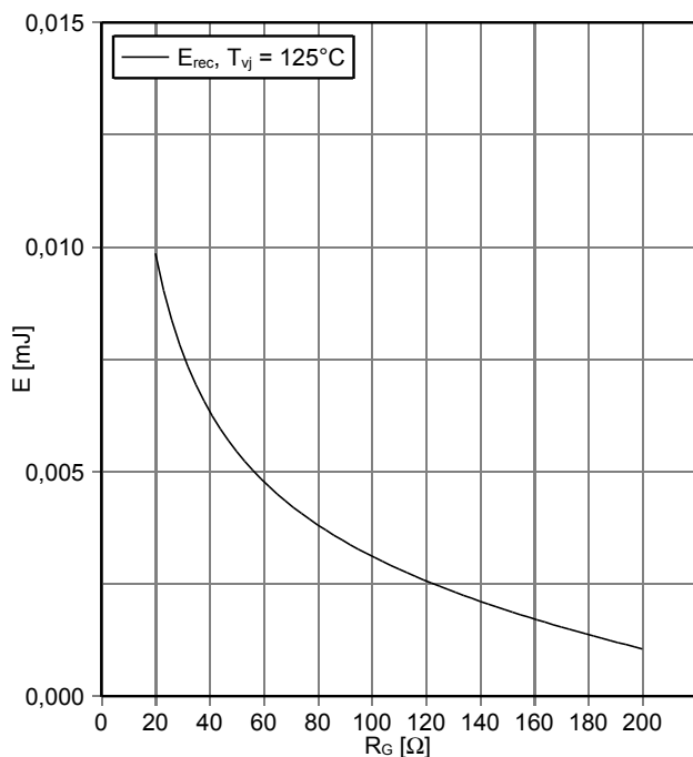
开关损耗 二极管, 三电平 (典型) switching losses Diode, 3-Level (typical) E_{rec} = f(R_G) I_F = 8 A, V_{CE} = 300 V
