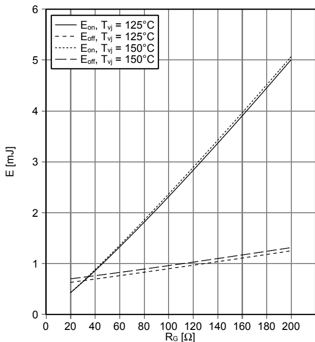
开关损耗 IGBT, 三电平 (典型) switching losses IGBT,3-Level (typical)
