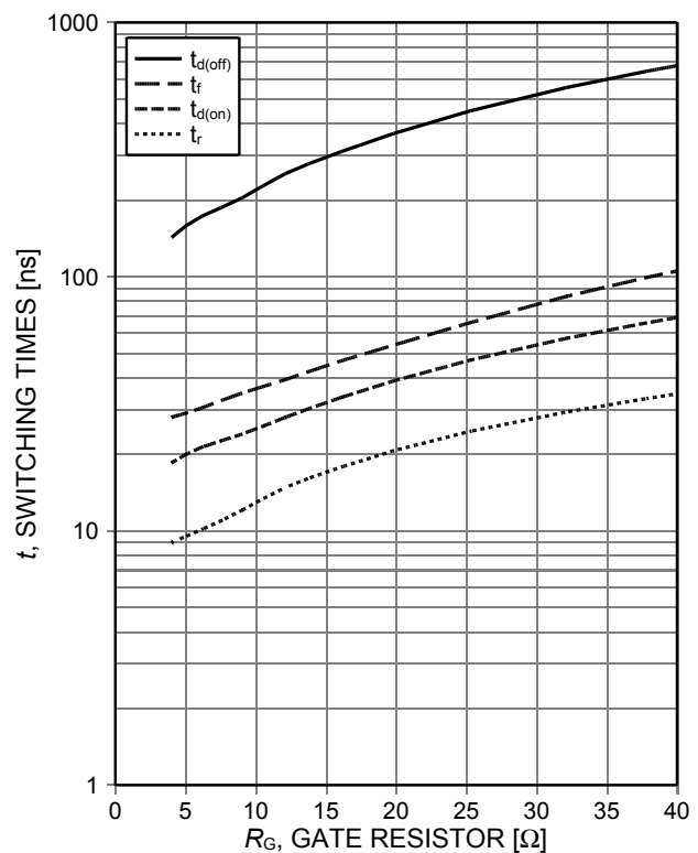
Figure 8. Typical switching times as a function of gate resistor (inductive load, T_{vj}=150^{\circ}C , V_{CE}=400V , V_{GE}=15/0V , I_C=37.5A , Dynamic test circuit in Figure E)
