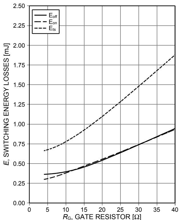
Figure 12. Typical switching energy losses as a function of gate resistor (inductive load, T_{vj}=150^\circ C , V_{CE}=400V , V_{GE}=15/0V , I_C=37.5A , Dynamic test circuit in Figure E)
