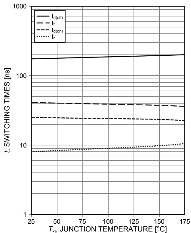
Figure 9. Typical switching times as a function of junction temperature (inductive load, V_{CE}=400V , V_{GE}=15/0V , I_C=37.5A , R_G=9\Omega , Dynamic test circuit in Figure E)
