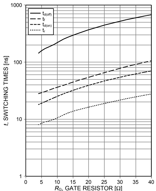
Figure 8. Typical switching times as a function of gate resistor (inductive load, T_J=150^{\circ}C , V_{CE}=400V , V_{GE}=15/0V , I_C=37.5A , Dynamic test circuit in Figure E)
