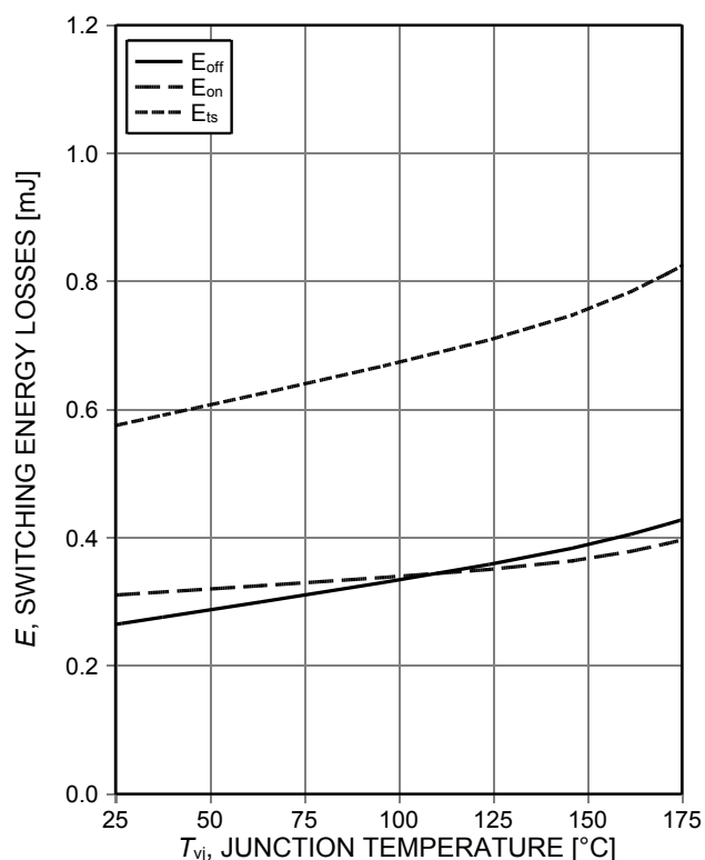
Figure 13. Typical switching energy losses as a function of junction temperature (inductive load, V_{CE}=400V , V_{GE}=15/0V , I_C=37.5A , R_G=9\Omega , Dynamic test circuit in Figure E)
