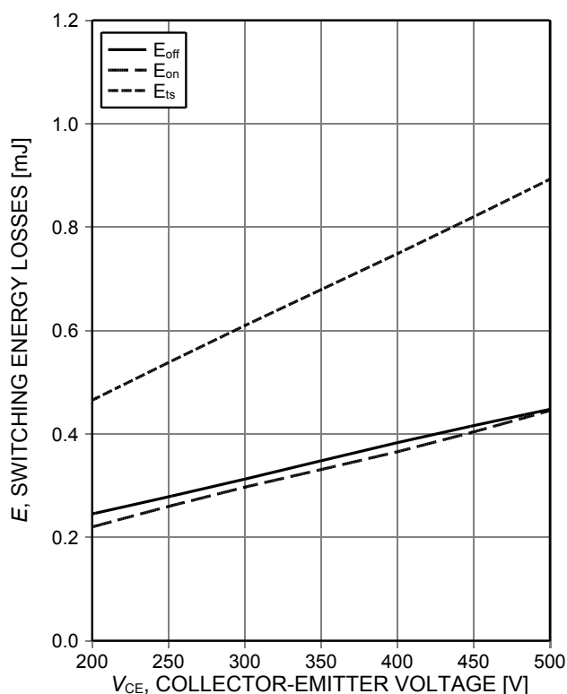
Figure 14. Typical switching energy losses as a function of collector emitter voltage (inductive load, T_{vj}=150^\circ C , V_{GE}=15/0V , I_C=37.5A , R_G=9\Omega , Dynamic test circuit in Figure E)
