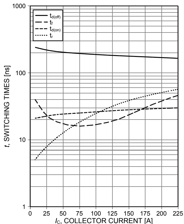
Figure 7. Typical switching times as a function of collector current (inductive load, T_J=150^{\circ}C , V_{CE}=400V , V_{GE}=15/0V , R_G=9\Omega , Dynamic test circuit in Figure E)
