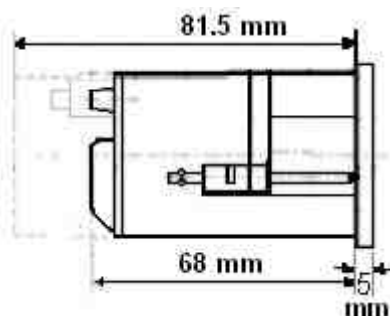
Mounting Position
