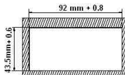
Installation Cutout
