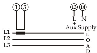
1PH Network
