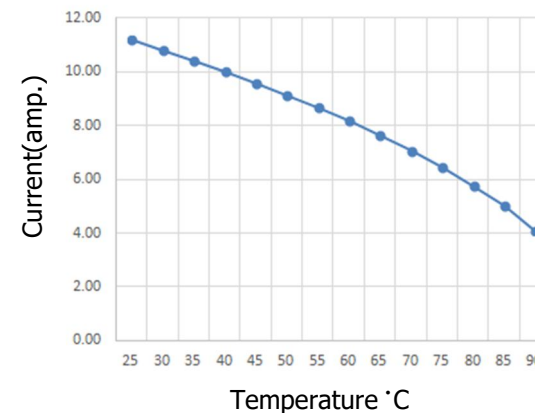
Derating curve
