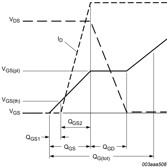
Fig. 17. Gate charge waveform definitions
