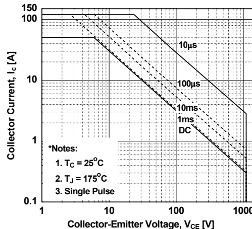
Figure 10. SOA Characteristics
