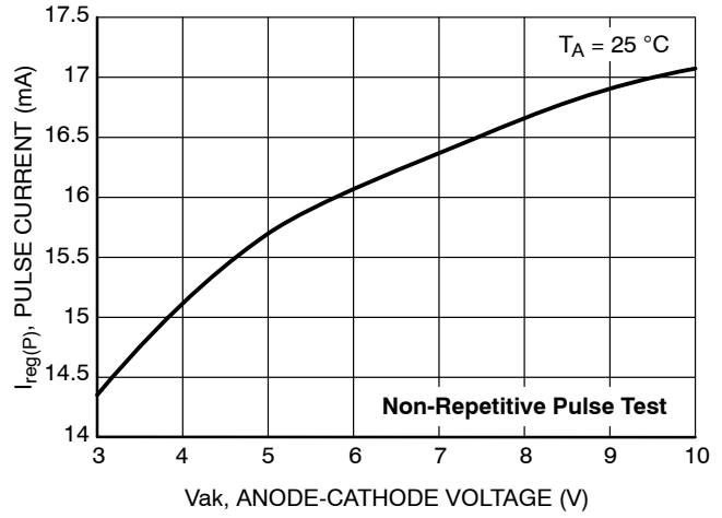
Figure 3. Pulse Current ( I_{\text{reg(P)}} ) vs. Anode-Cathode Voltage ( V_{\text{ak}} )
