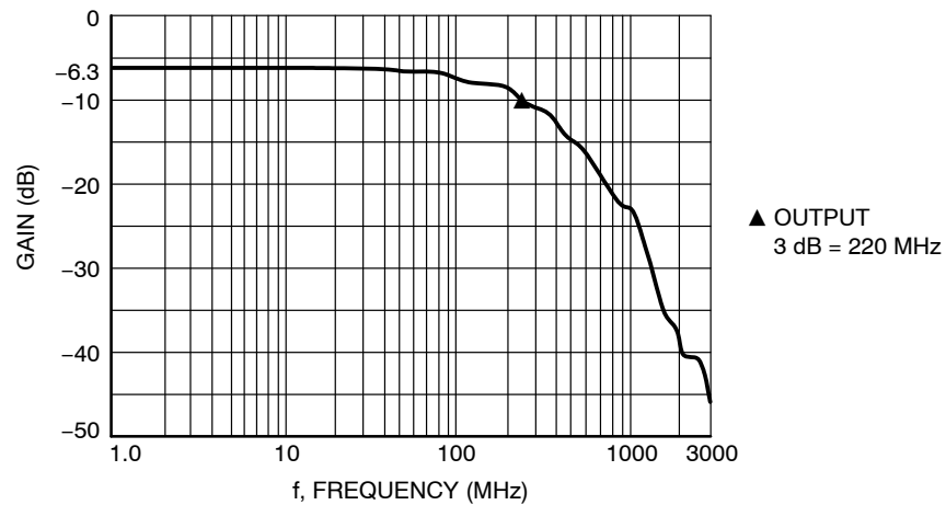
Figure 2. Typical EMI Filter Response (50 Ω Source and 50 Ω Load Termination)
