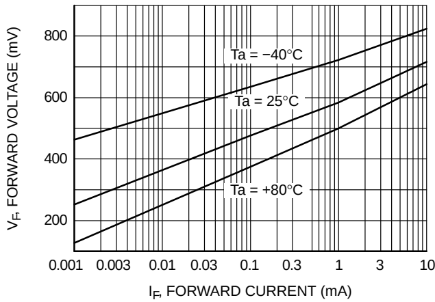
Figure 7. Forward Voltage vs. Ambient Temperature VF – 1.0 \mu\text{A} – 10 mA (– 40 to +80^\circ\text{C} )
