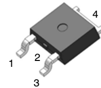
DPAK3 (TO-252 3 LD) CASE 369AS
