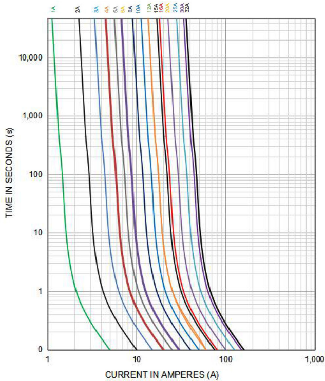
Average Current Curve(I-T Curve)
