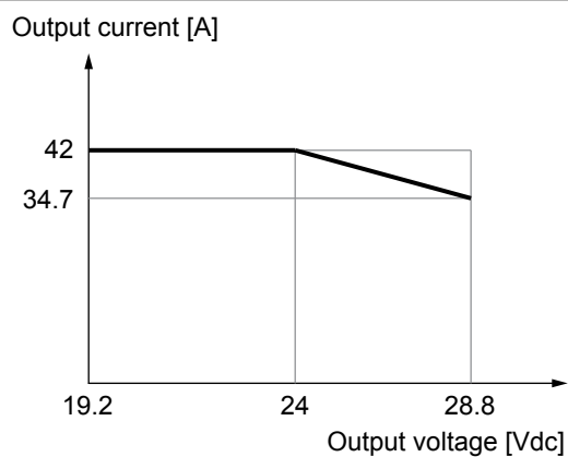
Fig. 10: Output current versus output voltage 24 V
