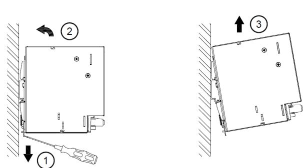
Fig. 2.2 Dismounting
