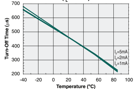
Typical Turn-Off Time vs. Temperature ( I_L=50\text{mA} )
