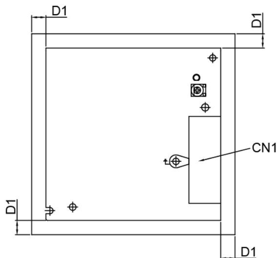
Fig. 3 Assembly Reference
