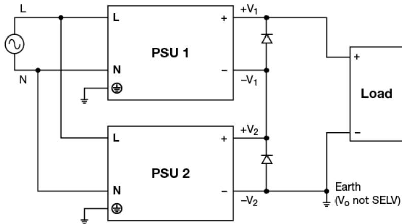
Fig. 5 Series Operation Connection Diagram
