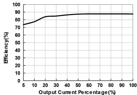
VXO7805-500-M Efficiency Curve Efficiency vs. Load Current (Vin = 24 V)
