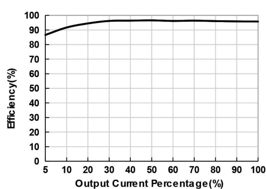
VXO78015-500-M Efficiency Curve Efficiency vs. Load Current (Vin = 24 V)
