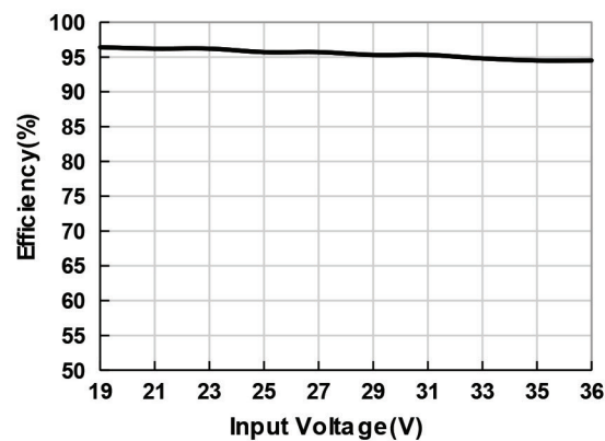
VXO78015-500-M Efficiency Curve Efficiency vs. Input Voltage (at full load)
