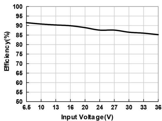
VXO7805-500-M Efficiency Curve Efficiency vs. Input Voltage (at full load)
