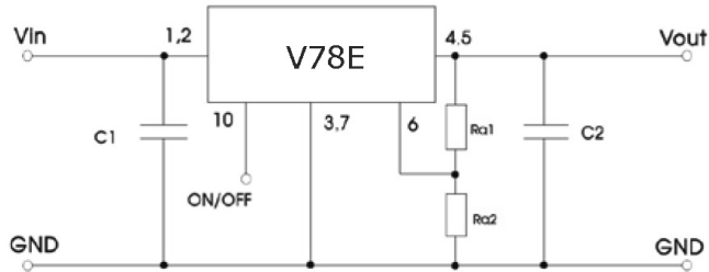
Application Circuit
