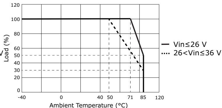
Temperature Derating Curves All Other Outputs (Natural Convection)
