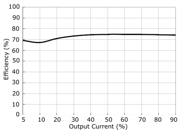
V78E01-1000-SMT Efficiency Curve Efficiency vs. Load Current (at V_{in} nominal)
