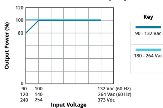
INPUT VOLTAGE DERATING CURVE (25°C)
