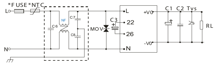
Figure 2 VSK-S3 EMC Filtering Circuit
