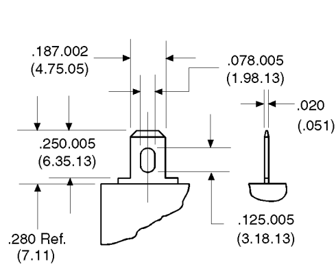
Solder/Plug In .187 Quick Connect
