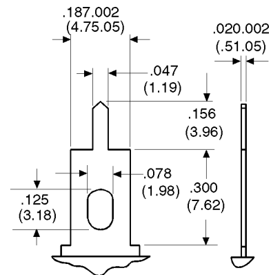
Printed Circuit Terminal
