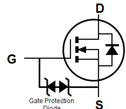
Equivalent Circuit
