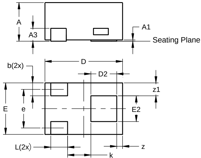
X2-DFN0604-3
