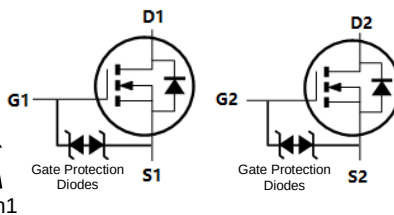
Internal Schematic
