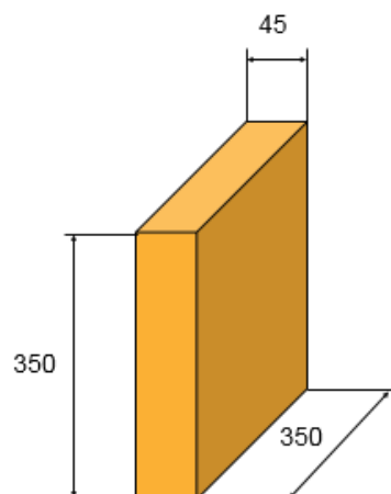
Figure 18. Inner box dimensions (mm)
