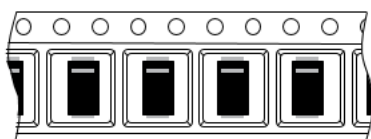
Figure 15. Package orientation in reel
