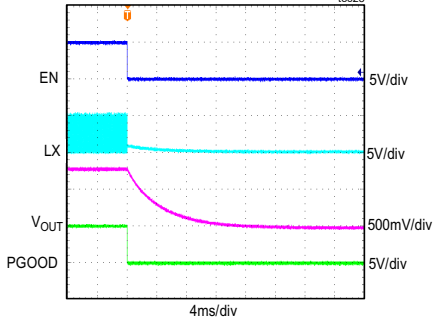
MAXM17623 SHUTDOWN THROUGH ENABLE ( V_{IN} = 5V , V_{OUT} = 0.8V , I_{LOAD} = 0A , PWM MODE)
