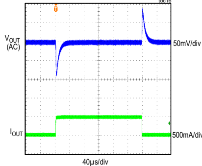
MAXM17624 LOAD TRANSIENT RESPONSE ( V_{IN} = 5V , V_{OUT} = 3.3V , PWM MODE) (LOAD CURRENT STEPPED FROM 0A TO 0.5A)
