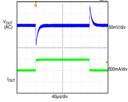
MAXM17624 LOAD TRANSIENT RESPONSE ( V_{IN} = 5V , V_{OUT} = 3.3V , PWM MODE) (LOAD CURRENT STEPPED FROM 0.5A TO 1A)
