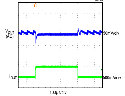
MAXM17623 LOAD TRANSIENT RESPONSE ( V_{IN} = 5V , V_{OUT} = 1.5V , PFM MODE) (LOAD CURRENT STEPPED FROM 0A TO 0.5A)
