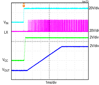
MAXM15464 STARTUP THROUGH V_{IN} V_{IN} = 24V , FIXED V_{OUT} = 5V , FULL LOAD, PWM MODE
