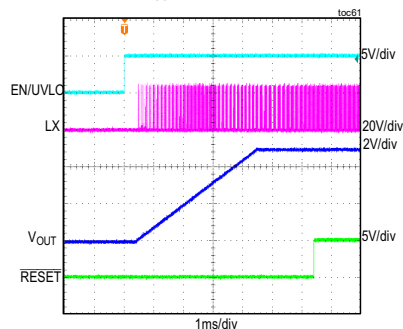
MAXM15464 STARTUP THROUGH ENABLE
