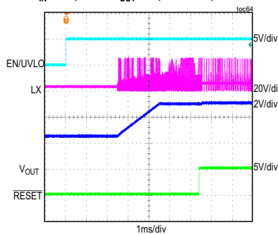
MAXM15464 STARTUP THROUGH ENABLE (2.5V PREBIAS) V_{IN} = 24V , FIXED V_{OUT} = 5V , NO LOAD, PFM MODE
