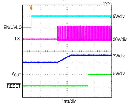
MAXM15462 STARTUP THROUGH ENABLE 2V PREBIAS, V_{IN} = 24V , ADJUSTABLE V_{OUT} = 3.3V , NO LOAD, PFM MODE
