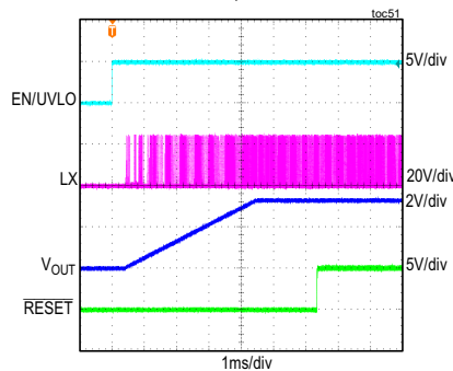
MAXM15462 STARTUP THROUGH ENABLE V_{IN} = 24V , ADJUSTABLE V_{OUT} = 3.3V , FULL LOAD, PWM MODE
