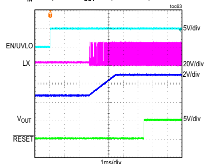
MAXM15464 STARTUP THROUGH ENABLE (2.5V PREBIAS)
