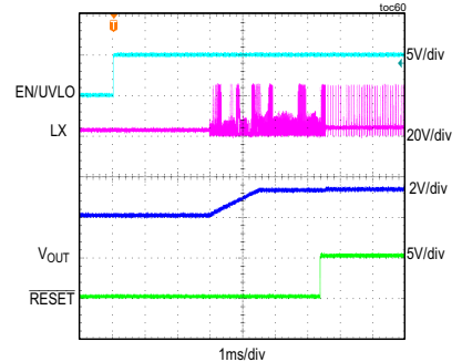
MAXM15463 STARTUP THROUGH ENABLE (2V PREBIAS)
