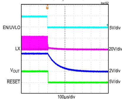
MAXM15462 SHUTDOWN THROUGH ENABLE V_{IN} = 24V , ADJUSTABLE V_{OUT} = 3.3V , FULL LOAD, PWM MODE
