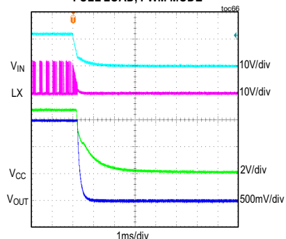
MAXM15462 SHUTDOWN THROUGH V_{IN} V_{IN} = 12V , ADJUSTABLE V_{OUT} = 1.5V , FULL LOAD, PWM MODE
