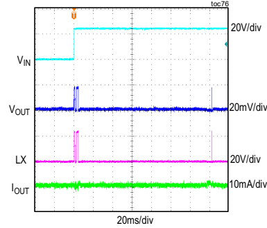
MAXM15462 OUTPUT SHORT DURING STARTUP V_{IN} = 24V , V_{OUT} = 3.3V , FULL LOAD, PWM MODE
