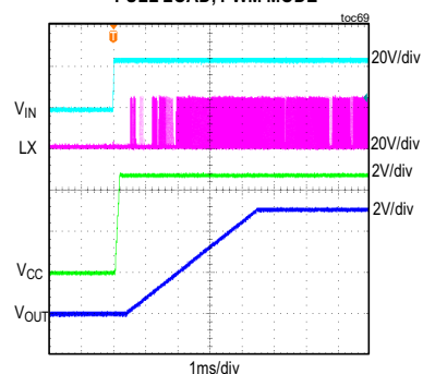
MAXM15462 STARTUP THROUGH V_{IN} V_{IN} = 24V , ADJUSTABLE V_{OUT} = 5V , FULL LOAD, PWM MODE
