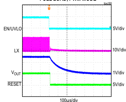
MAXM15462 SHUTDOWN THROUGH ENABLE V_{IN} = 12V , ADJUSTABLE V_{OUT} = 1.5V , FULL LOAD, PWM MODE
