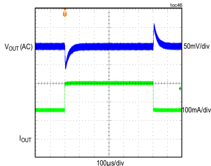
MAXM15463 LOAD TRANSIENT RESPONSE V_{IN} = 24V , FIXED V_{OUT} = 3.3V , PWM MODE (LOAD CURRENT STEPPED FROM 150mA TO 300mA)
