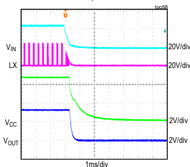
MAXM15462 SHUTDOWN THROUGH V_{IN} V_{IN} = 24V , ADJUSTABLE V_{OUT} = 3.3V , FULL LOAD, PWM MODE
