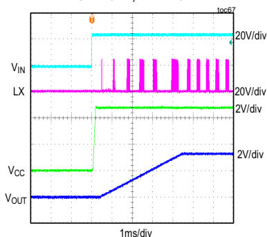
MAXM15462 STARTUP THROUGH V_{IN} V_{IN} = 24V , ADJUSTABLE V_{OUT} = 3.3V , FULL LOAD, PWM MODE
