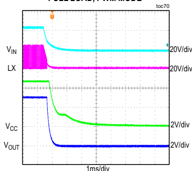
MAXM15462 SHUTDOWN THROUGH V_{IN} V_{IN} = 24V , ADJUSTABLE V_{OUT} = 5V , FULL LOAD, PWM MODE
