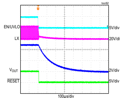
MAXM15464 SHUTDOWN THROUGH ENABLE
