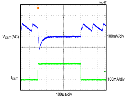
MAXM15464 LOAD TRANSIENT RESPONSE V_{IN} = 24V , FIXED V_{OUT} = 5V , PFM MODE (LOAD CURRENT STEPPED FROM 5mA TO 150mA)
