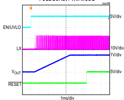
MAXM15462 STARTUP THROUGH ENABLE V_{IN} = 12V , ADJUSTABLE V_{OUT} = 1.5V , FULL LOAD, PWM MODE
