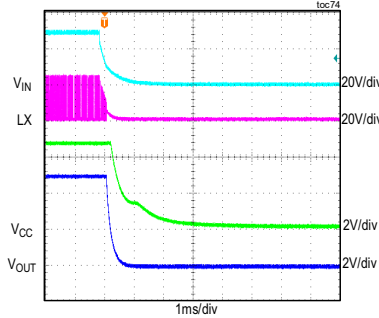
MAXM15464 SHUTDOWN THROUGH V_{IN} V_{IN} = 24V , FIXED V_{OUT} = 5V , FULL LOAD, PWM MODE
