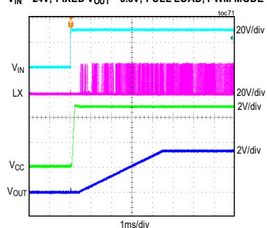
MAXM15463 STARTUP THROUGH V_{IN} V_{IN} = 24V , FIXED V_{OUT} = 3.3V , FULL LOAD, PWM MODE
