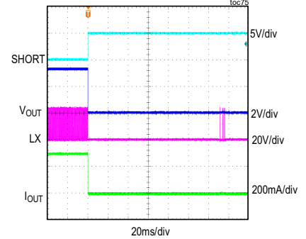
MAXM15462 OUTPUT SHORT IN STEADY STATE V_{IN} = 24V , ADJUSTABLE V_{OUT} = 3.3V , FULL LOAD, PWM MODE
