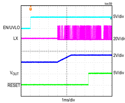
MAXM15463 STARTUP THROUGH ENABLE (2V PREBIAS)
