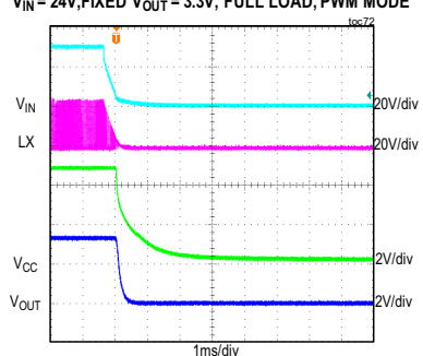
MAXM15463 SHUTDOWN THROUGH V_{IN} V_{IN} = 24V , FIXED V_{OUT} = 3.3V , FULL LOAD, PWM MODE
