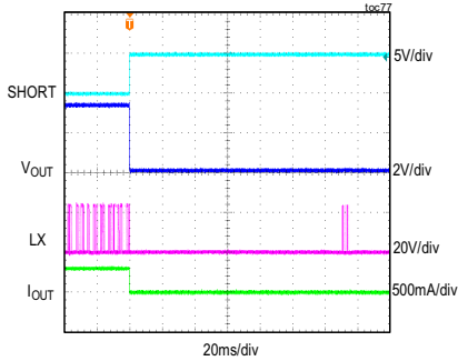
MAXM15463 OUTPUT SHORT IN STEADY STATE V_{IN} = 24V , FIXED V_{OUT} = 3.3V , FULL LOAD, PWM MODE
