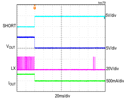
MAXM15464 OUTPUT SHORT IN STEADY STATE V_{IN} = 24V , FIXED V_{OUT} = 5V , FULL LOAD, PWM MODE
