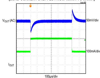
MAXM15464 LOAD TRANSIENT RESPONSE V_{IN} = 24V , FIXED V_{OUT} = 5V , PWM MODE (LOAD CURRENT STEPPED FROM 150mA TO 300mA)
