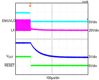
MAXM15463 SHUTDOWN THROUGH ENABLE
