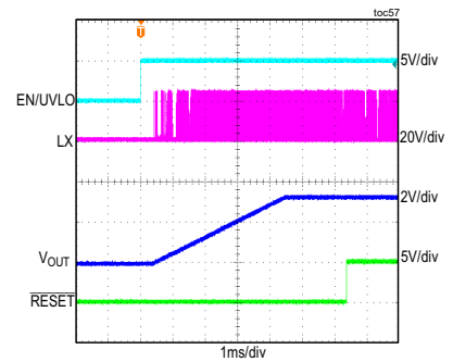
MAXM15463 STARTUP THROUGH ENABLE
