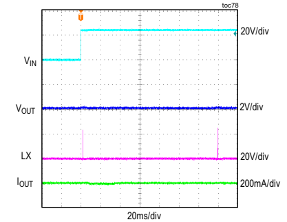
MAXM15463 OUTPUT SHORT DURING STARTUP V_{IN} = 24V , FIXED V_{OUT} = 3.3V , FULL LOAD, PWM MODE
