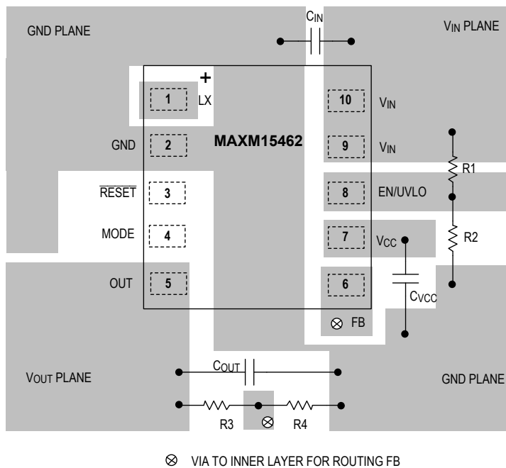
Figure 3. Adjustable Output Layout Guidelines
