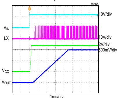
MAXM15462 STARTUP THROUGH V_{IN} V_{IN} = 12V , ADJUSTABLE V_{OUT} = 1.5V , FULL LOAD, PWM MODE
