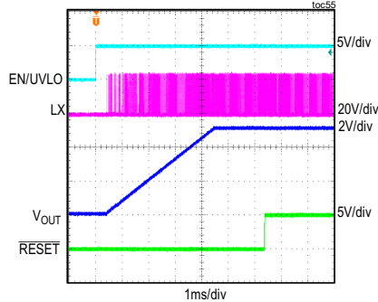
MAXM15462 STARTUP THROUGH ENABLE
