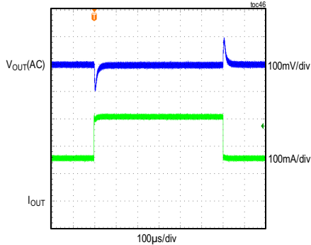
MAXM15067 LOAD TRANSIENT RESPONSE V_{IN} = 24V , ADJUSTABLE V_{OUT} = 3.3V , PWM MODE (LOAD CURRENT STEPPED FROM 150mA TO 300mA)
