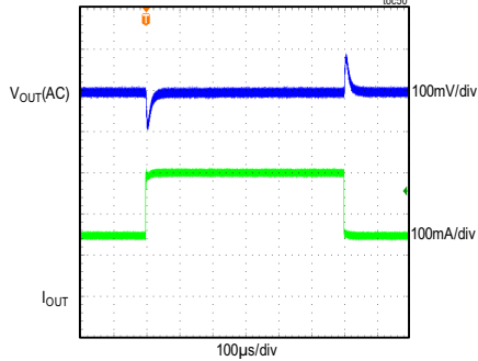
MAXM15065 LOAD TRANSIENT RESPONSE V_{IN} = 24V , FIXED V_{OUT} = 3.3V , PWM MODE (LOAD CURRENT STEPPED FROM 150mA TO 300mA)
