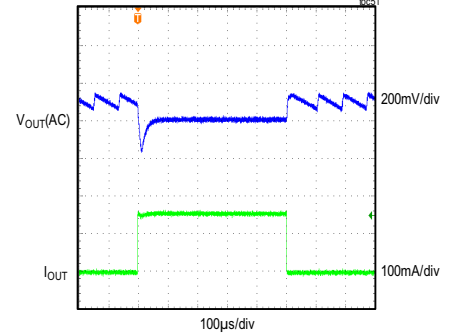
MAXM15066 LOAD TRANSIENT RESPONSE V_{IN} = 24V , FIXED V_{OUT} = 5V , PFM MODE (LOAD CURRENT STEPPED FROM 5mA TO 150mA)
