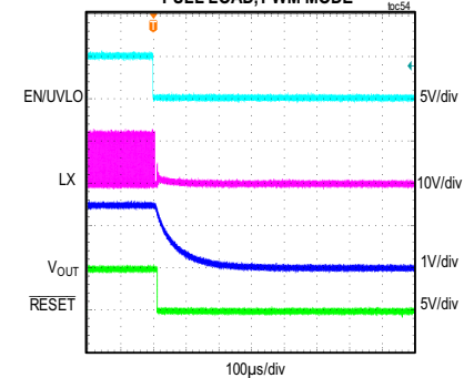
MAXM15067 SHUTDOWN THROUGH ENABLE V_{IN} = 12V , ADJUSTABLE V_{OUT} = 1.5V , FULL LOAD, PWM MODE
