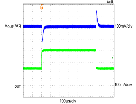
MAXM15067 LOAD TRANSIENT RESPONSE V_{IN} = 24V , ADJUSTABLE V_{OUT} = 5V , PWM MODE (LOAD CURRENT STEPPED FROM 150mA TO 300mA)
