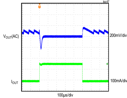
MAXM15067 LOAD TRANSIENT RESPONSE V_{IN} = 24V , ADJUSTABLE V_{OUT} = 5V , PFM MODE (LOAD CURRENT STEPPED FROM 5mA TO 150mA)
