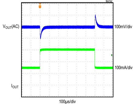
MAXM15066 LOAD TRANSIENT RESPONSE V_{IN} = 24V , FIXED V_{OUT} = 5V , PWM MODE (LOAD CURRENT STEPPED FROM 150mA TO 300mA)
