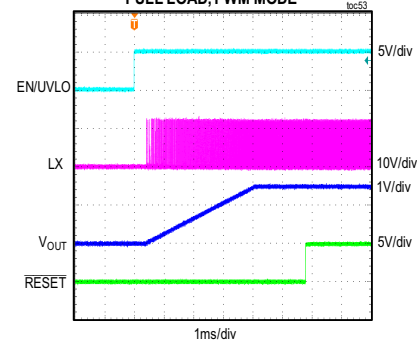
MAXM15067 STARTUP THROUGH ENABLE V_{IN} = 12V , ADJUSTABLE V_{OUT} = 1.5V , FULL LOAD, PWM MODE
