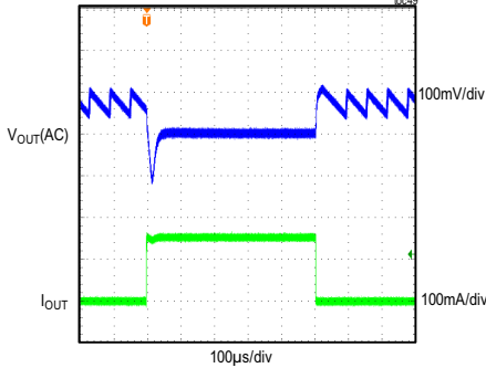
MAXM15065 LOAD TRANSIENT RESPONSE V_{IN} = 24V , FIXED V_{OUT} = 3.3V , PFM MODE (LOAD CURRENT STEPPED FROM 5mA TO 150mA)
